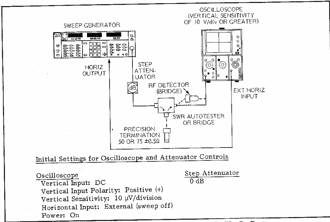
Figure 3-2. Equipment Setup for Direct, Go/No-Go Test
