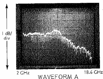
Bad center-pin mating between air line and SWR Autotester
